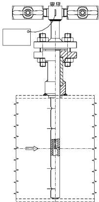
Fixed type not extractable from pipe Threaded process connection
